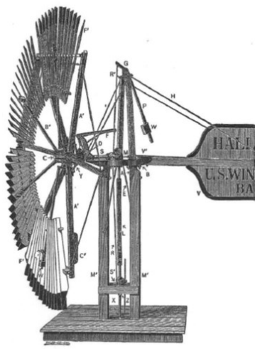
The Improved Halladay Standard Pumping Wind Mill.
